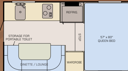
80SK Fits short or long bed trucks
