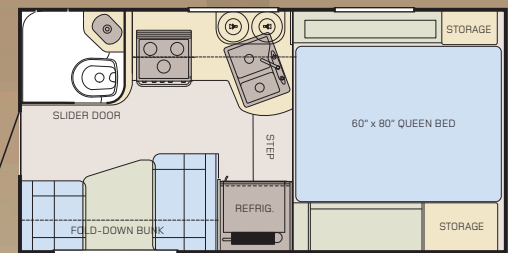
NEW 89RB Fits short or long bed
