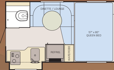
80GS Fits short bed trucks only
